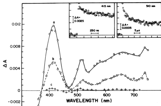
Figure 21. Transient difference absorption spectra obtained upon 532-nm laser pulse excitation of aqueous solutions of \text{RuL}_3^{4-} (40 \mu\text{M} ) and \text{ABTS}^{2-} (100 \mu\text{M} ) with (spectra a and b) and without (spectrum c) \text{SiO}_2/\text{Al}_2\text{O}_3 particles (3.7 g/L). Spectrum a was obtained immediately and spectra b and c were recorded with a 25- \mu\text{s} delay. The insets show the kinetic traces recorded at 415 and 510 nm of the sample containing \text{SiO}_2/\text{Al}_2\text{O}_3 particles. Reprinted from ref 67. Copyright 1989 American Chemical Society.
