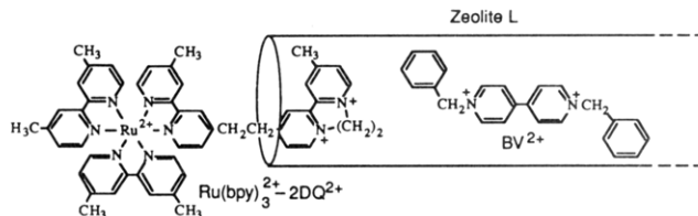
Figure 22. A zeolite-based compartmentalized photochemical system. (T. Mallouk, private communication.)
