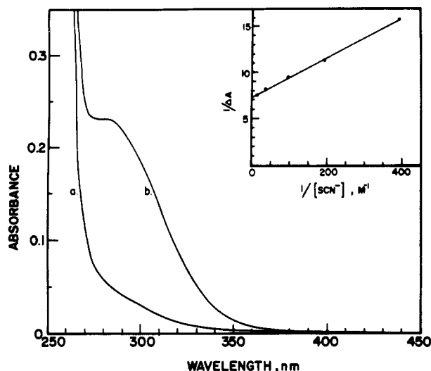
Figure 27. Absorption spectra of (a) 0.005 M SCN - (vs acetonitrile as reference) and 0.005 M SCN - and 28 μM TiO 2 (vs 28 μM TiO 2 in acetonitrile as reference). Insert shows the Benesi-Hildebrand plot for the determination of the apparent association constant for the association between TiO 2 and SCN - . Reprinted from ref 60. Copyright 1985 American Chemical Society.
