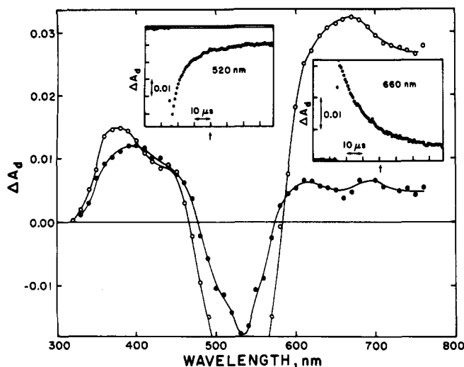
Figure 17. Transient absorption spectra of rose bengal dye on alumina (0.4 mg/g of \text{Al}_2\text{O}_3 ) recorded immediately after the 532-nm laser pulse excitation: (O) degassed and (●) air-equilibrated samples. (Inset show decay traces at 520 and 660 nm.) Reprinted from ref 39. Copyright 1989 American Chemical Society.
