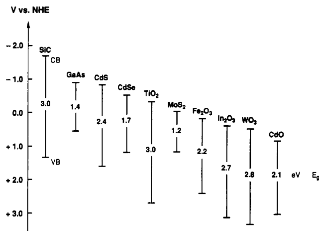
Figure 26. Bandgap energies and conduction and valence band energy levels of various semiconductors at pH 7.
