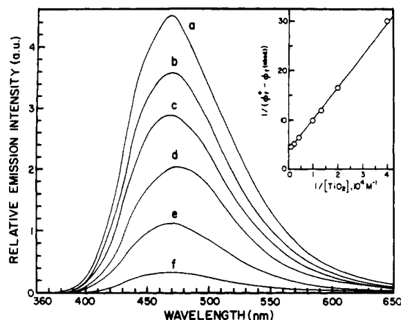
Figure 44. Fluorescence emission spectra of 20 mM anthracene-9-carboxylic acid in acetonitrile at various concentrations of \text{TiO}_2 : (a) 0, (b) 0.05, (c) 0.1, (d) 0.25, (e) 0.5, and (f) 1 mM. The excitation wavelength was at 355 nm, and the spectra were corrected for the photomultiplier response. Insert shows the dependence of 1/(\phi_f^0 - \phi_f(\text{obsd})) on the reciprocal concentration of \text{TiO}_2 (see eq 28 for details). Reprinted from ref 57. Copyright 1989 American Chemical Society.
