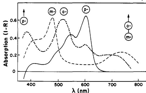
Figure 16. Diffuse reflectance transient absorption spectra of o -, m -, and p -DSB adsorbed on silica ( c = 7 \times 10^{-7} \text{ mol g}^{-1} , T = 293 \text{ K} ), recorded with a 50- \mu\text{s} delay after laser pulse excitation at 354 nm. Reprinted from ref 122. Copyright 1988 American Chemical Society.
