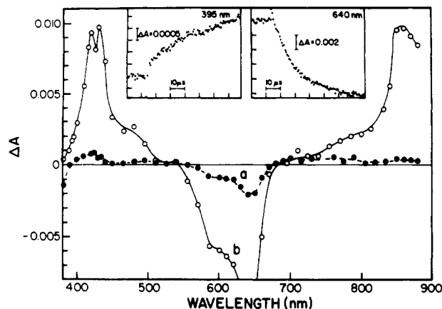
Figure 52. Sensitized reduction of Ox725. Transient absorption spectra recorded upon 355-nm laser pulse excitation of 20 \mu\text{M} 9AC and 5 \text{ mM} Ox725: (a, ●) in acetonitrile and (b, ○) in acetonitrile containing 2 \text{ mM} \text{TiO}_2 . The spectra were recorded 110 \mu\text{s} after the laser pulse excitation. Inserts show the formation of \text{Ox}^- (395 nm) and depletion of Ox725 (640 nm) in \text{TiO}_2 suspensions. Reprinted from ref 57. Copyright 1989 American Chemical Society.
