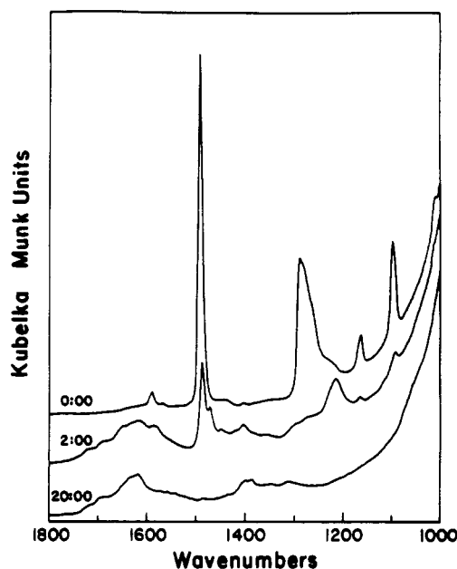
Figure 42. Diffuse reflectance FTIR spectra recorded during the photodegradation of 4-chlorophenol adsorbed on TiO 2 . The samples were analyzed following the UV irradiation for (a) 0, (b) 2, and (c) 20 h. Spectrum a corresponds to the chemisorbed chlorophenol, spectrum b corresponds to the reaction intermediates (e.g., hydroquinone), and spectrum c shows the disappearance of organic molecules bound to the TiO 2 surface. Reprinted from ref 482. Copyright 1992 Elsevier Science Publishers, B. V.
