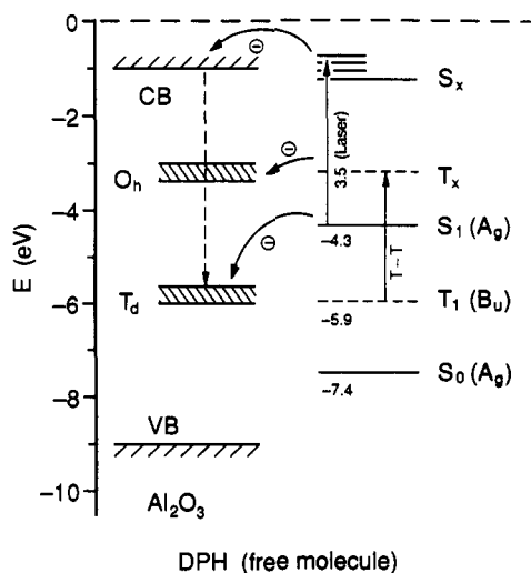
Figure 18. Energy level diagram of alumina showing the positions of the valence band (VB) and conduction band (CB) and including the approximate energies of the Al surface centers with T_d and O_h coordination. The energy levels of DPH relative to its ionization potential are also shown. Reprinted from ref 122. Copyright 1988 American Chemical Society.
