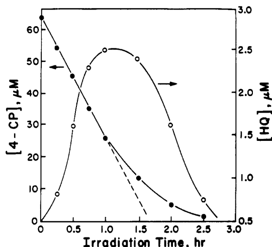
Figure 41. Degradation of 4-CP (●) and the formation and degradation of HQ (○) as a function of irradiation time. Initial [4-CP] = 63 μM. Other conditions are as follows: initial pH, 5.85; flow rate, 250 mL min -1 ; temperature, 30 ± 2 °C. Reprinted from ref 478b. Copyright 1989 American Chemical Society.
