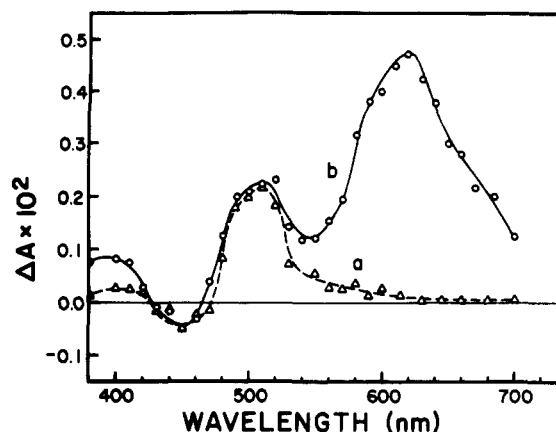
Figure 38. Formation of \text{Et}_2\text{NCS}_2 in colloidal CdS suspension. Transient absorption spectra recorded immediately after the 355-nm laser pulse excitation of 0.2 mM colloidal CdS in acetonitrile containing (a) no \text{Et}_2\text{NCS}_2^- and (b) 2.5 mM \text{Et}_2\text{NCS}_2^- . Reprinted from ref 303. Copyright 1989 American Chemical Society.
