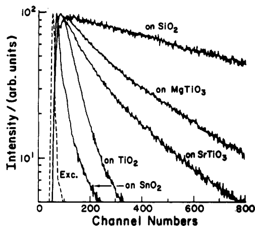
Figure 50. Fluorescence decays of Rh B adsorbed on metal oxide powders in vacuo (4.88 ps/channel). The excitation pulse (dotted line) shape is also shown. Reprinted from ref 495. Copyright 1988 Elsevier Science Publishers, B. V.
